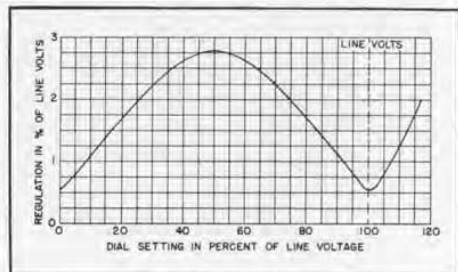
Figure 1. Percentage regulation as a function of output voltage for Variacs operated normally.
