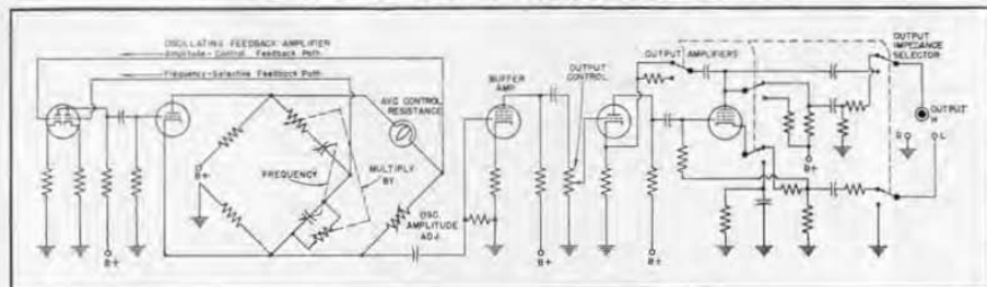
Figure 2. Elementary schematic circuit diagram of the oscillator.
