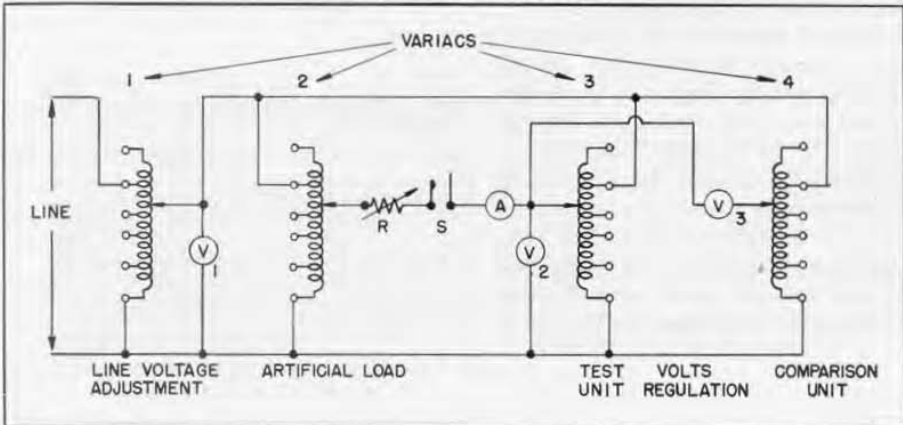
Figure 1. Circuit for regulation measurements.
